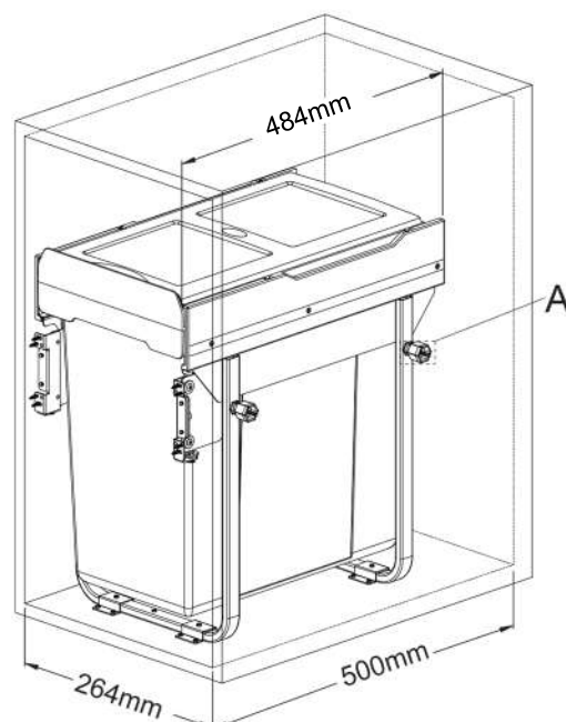
Minimum Cabinet Interior Dimension Requirements
