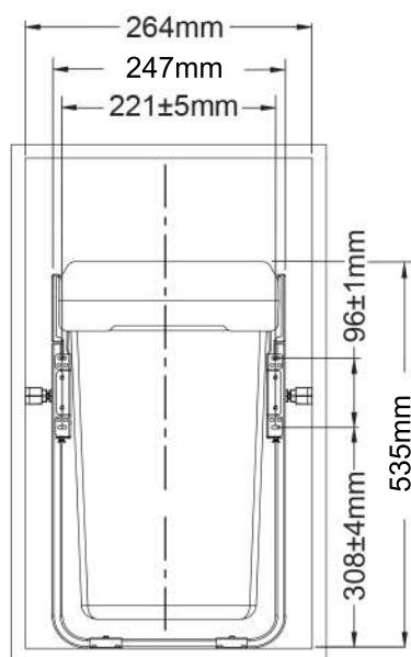
Unit Dimensions
